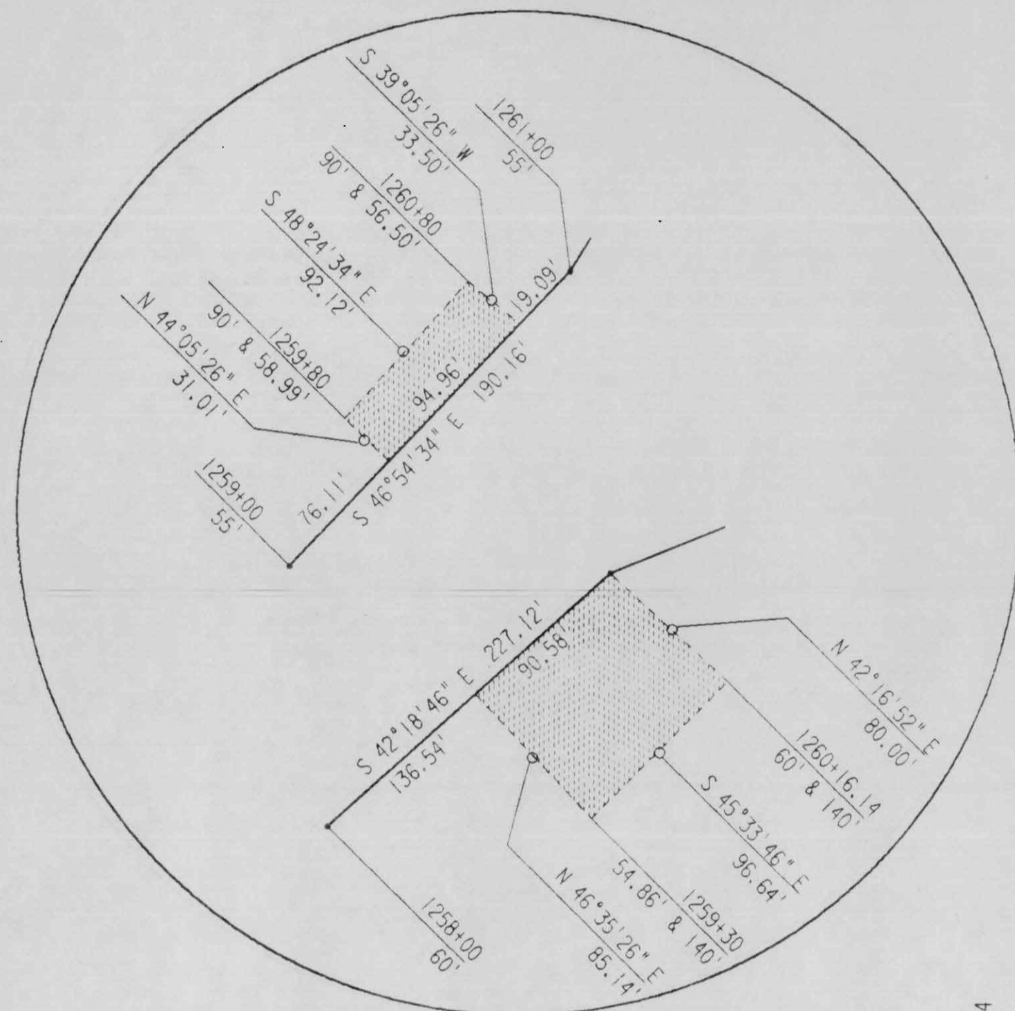
DETAIL A
