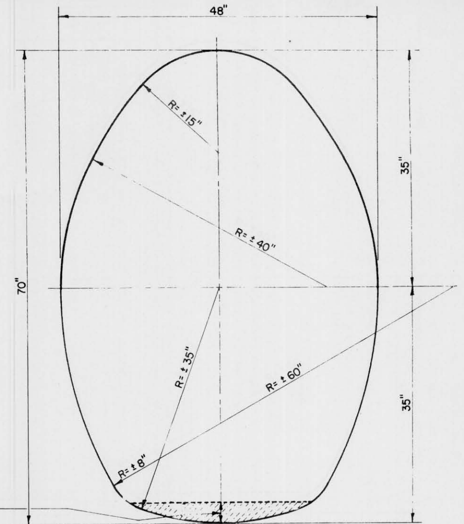
CORRUGATED GALVANIZED SHEET METAL PIPE CATTLE PASS NO. 10 GAUGE
