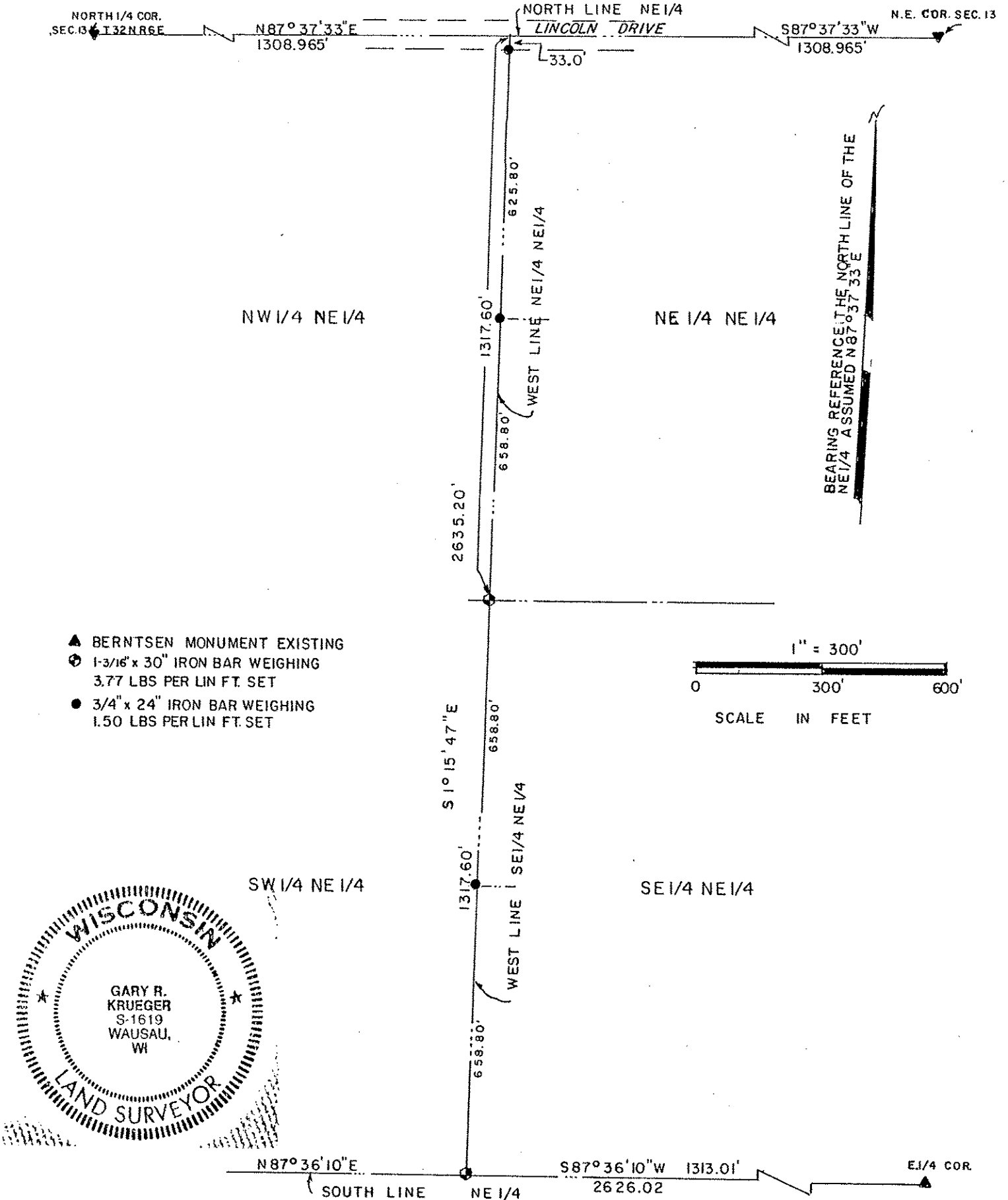
PLAT OF SURVEY MAP
