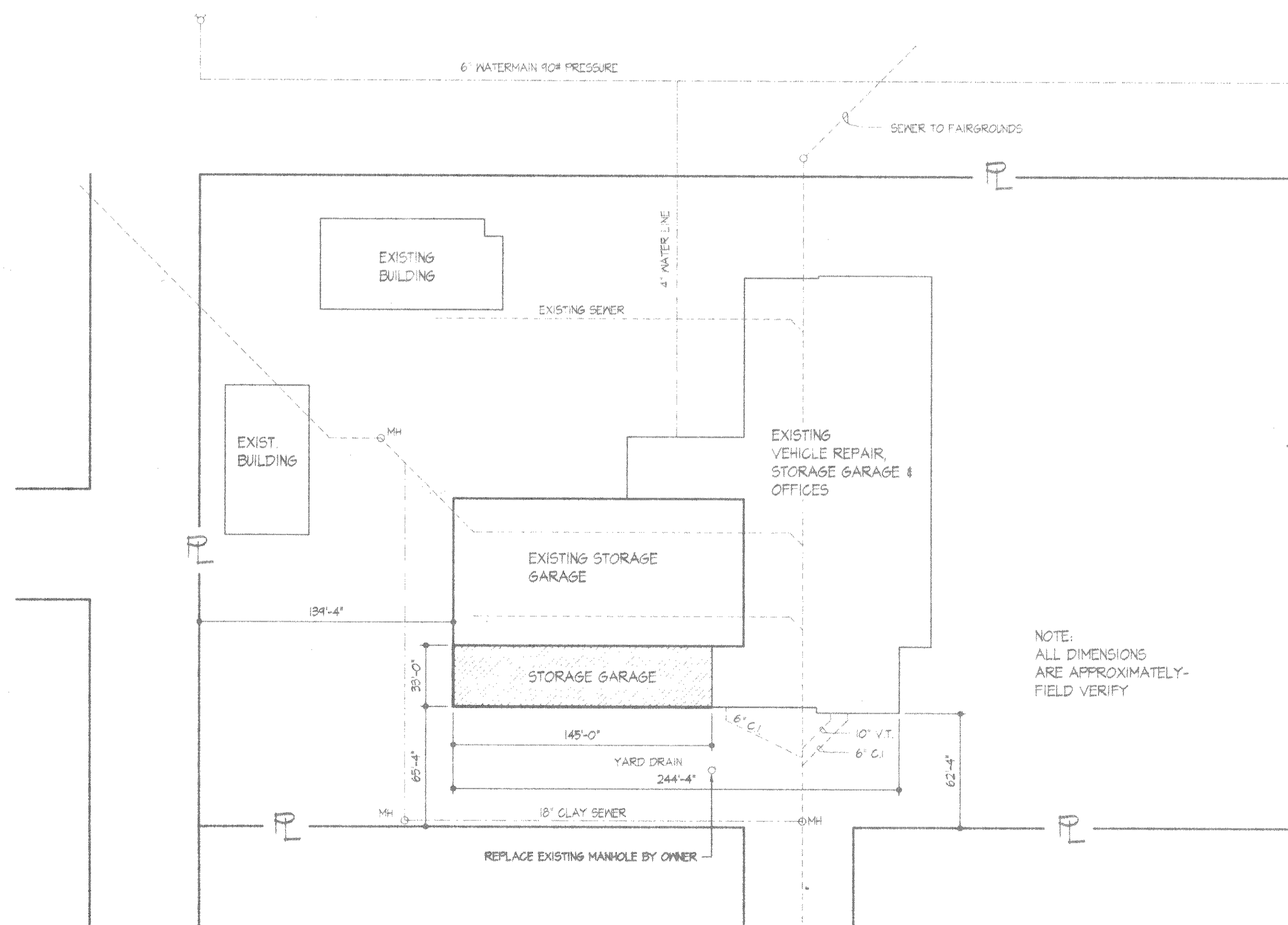
SITE PLAN SCALE: 1" = 50'-0"
