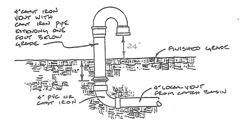
2 GOOSENECK DETAIL P-1 NO SCALE
