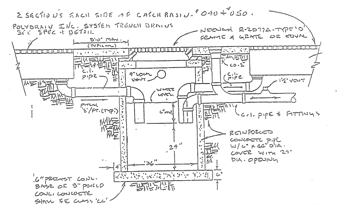
3 GARAGE CATCH BASIN DETAIL P-1 NO SCALE
