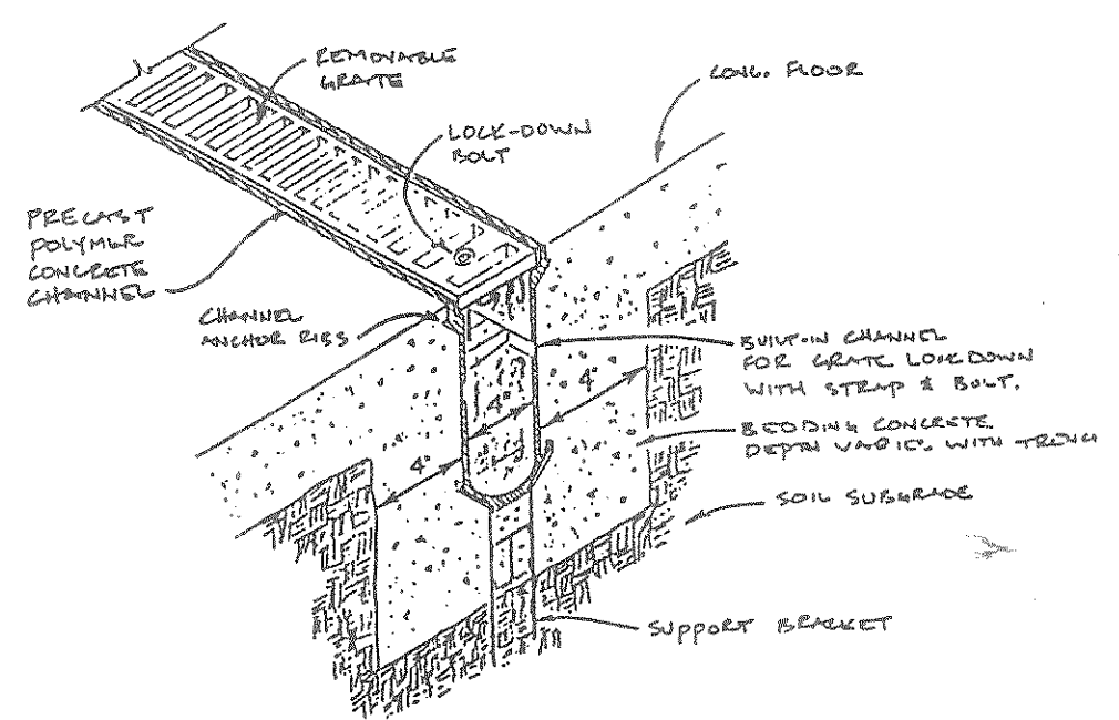
4 TRENCH DRAIN DETAIL P-1 NO SCALE
