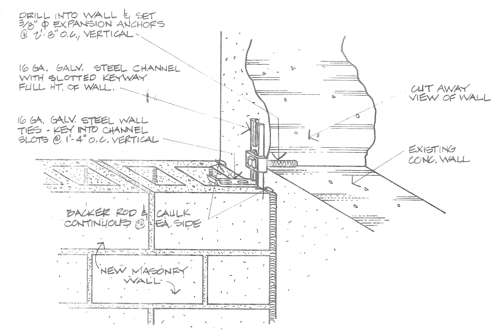
MASONRY ANCHORAGE DETAIL 3 A5 ISOMETRIC
