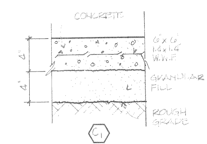
5 CONCRETE WALK 1/2" = 1'-0"
