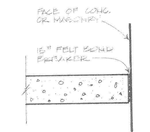
4 EXPANSION JOINT 1/2" = 1'-0"
