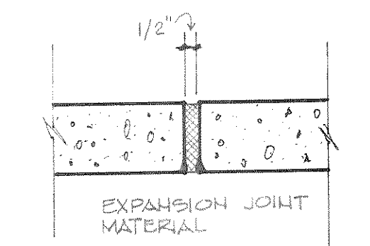
2 EXPANSION JOINT 1/2" = 1'-0"
