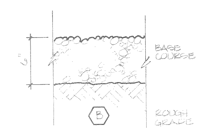
7 BASE COURSE 1/2" = 1'-0"
