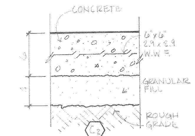
6 CONCRETE DRIVE 1/2" = 1'-0"
