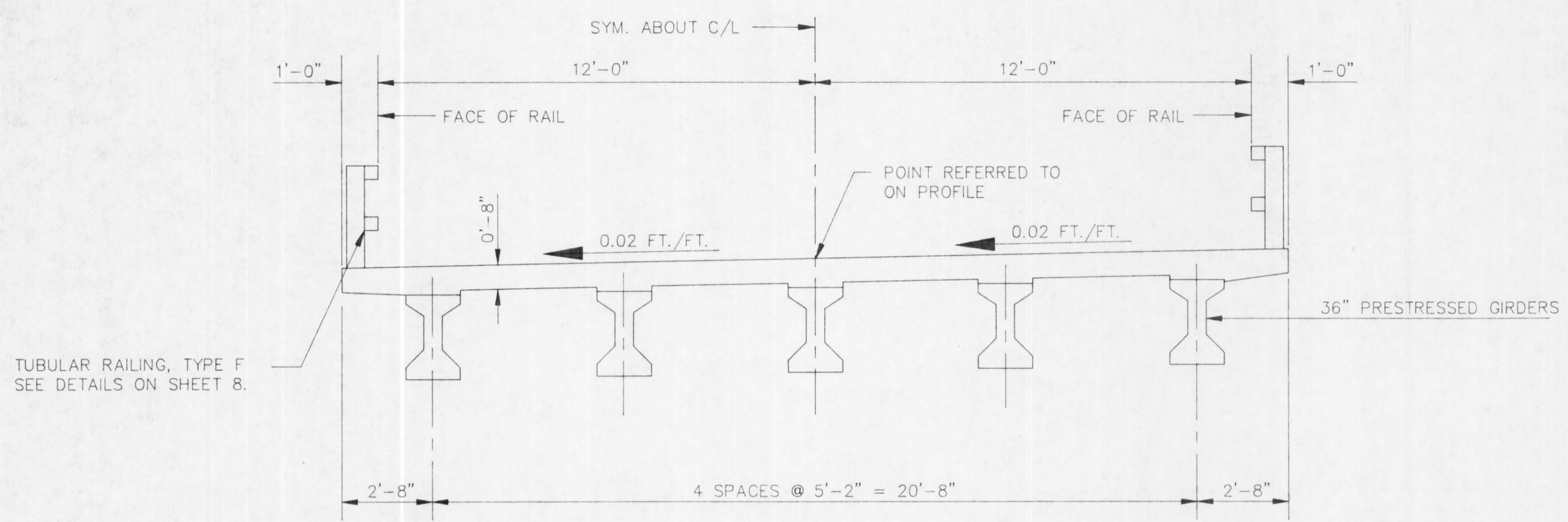
CROSS SECT. THRU RDWY.
