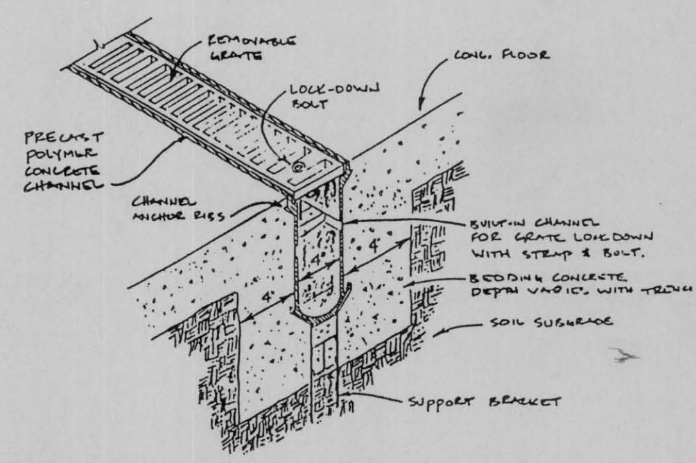
4 TRENCH DRAIN DETAIL NO SCALE P-1
