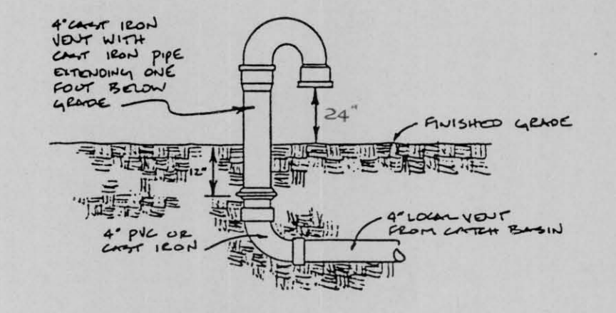
2 GOOSENECK DETAIL NO SCALE P-1
