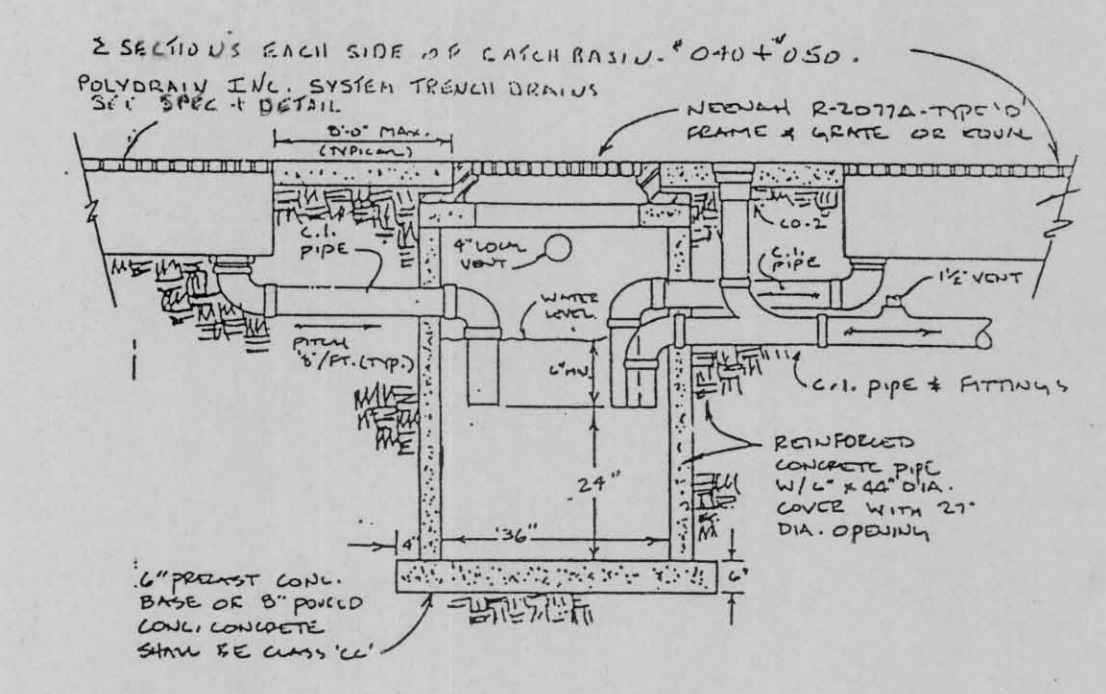
3 GARAGE CATCH BASIN DETAIL NO SCALE P-1
