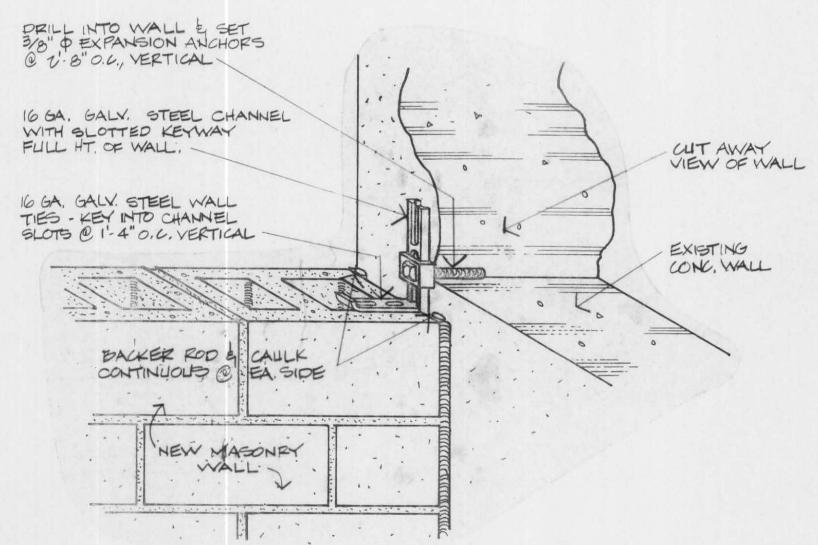
MASONRY ANCHORAGE DETAIL A5 ISOMETRIC
