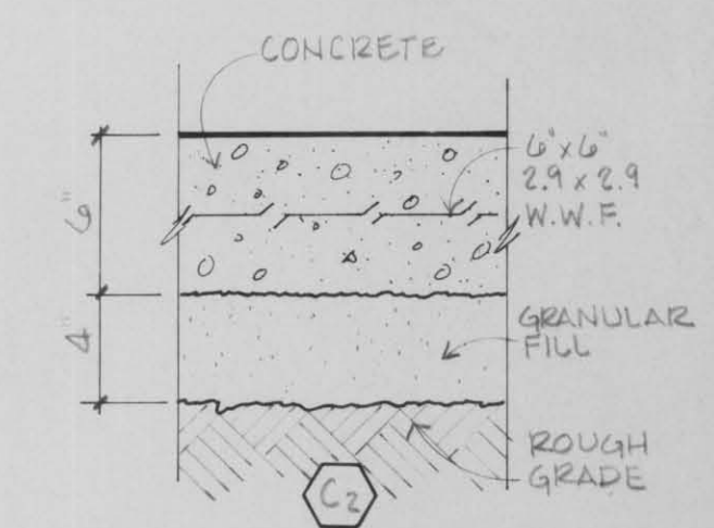
6 CONCRETE DRIVE 1/2" = 1'-0"
