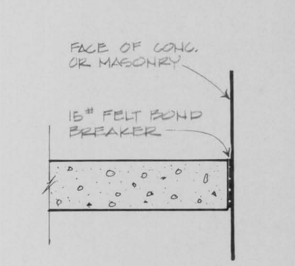
4 EXPANSION JOINT 1/2" = 1'-0"
