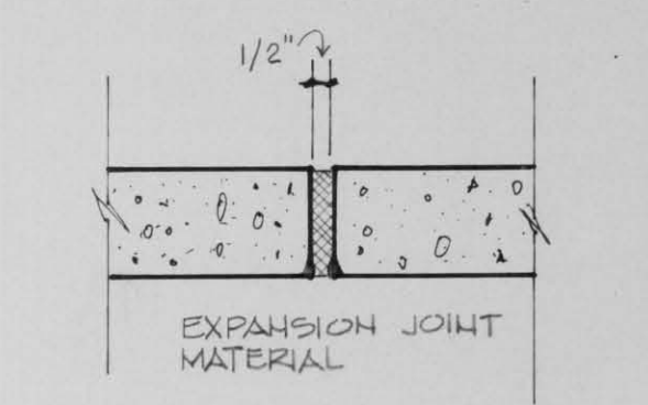
2 EXPANSION JOINT 1/2" = 1'-0"
