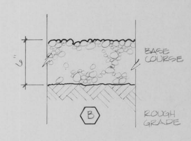
7 BASE COURSE 1/2" = 1'-0"
