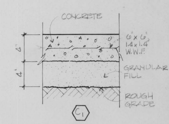
5 CONCRETE WALK 1/2" = 1'-0"
