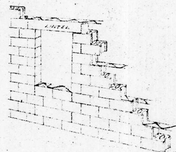
Detail of Wall Reinforcing
