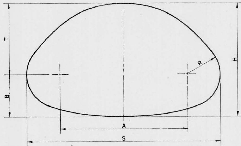
CORRUGATED GALVANIZED SHEET METAL PIPE ARCH (RIVETED)
