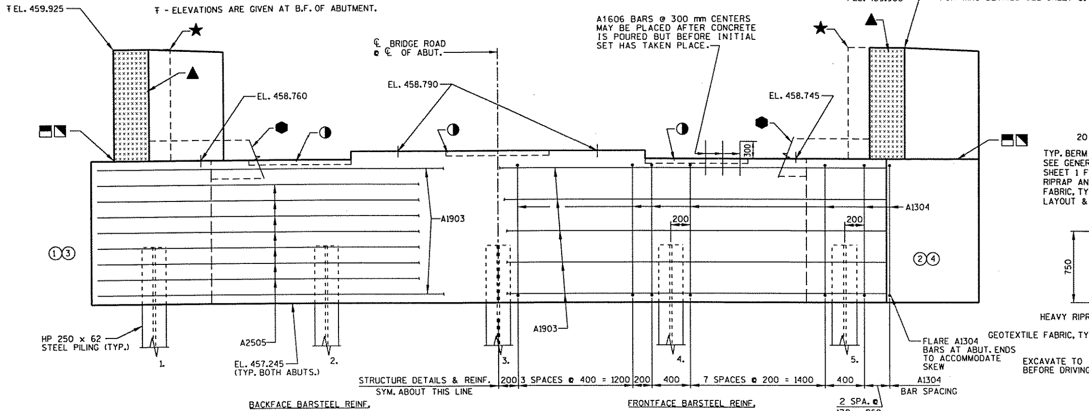
TYPICAL SECTION THRU ABUTMENT
