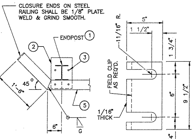
END DETAIL FOR WINGS
