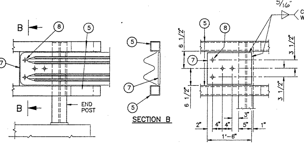
DETAIL AT END POST (PLATE BEAM GUARD RAIL ATTACHMENT)
