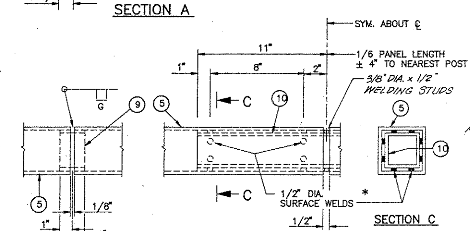
FIELD ERECTION JOINT DETAIL
