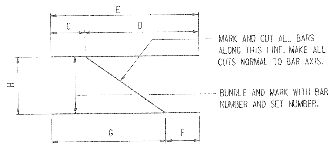
CUTTING DIAGRAM
